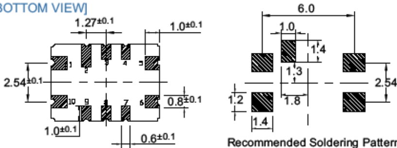
Recommended Soldering Pattern
