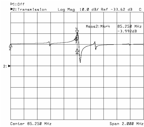
Horizontal: 0.2MHz/Div Vertical: 10dB/Div
