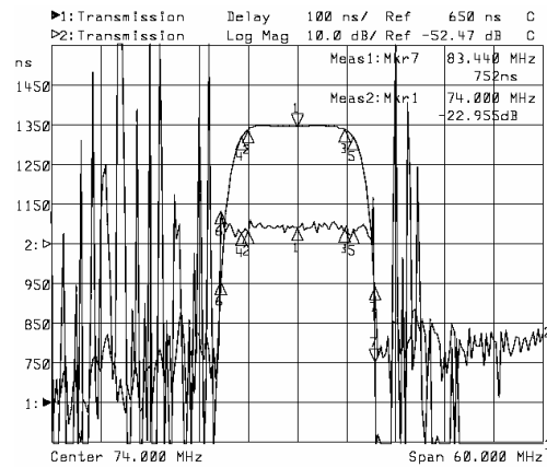
Horizontal: 6MHz/Div Vertical: 100nsec/Div
