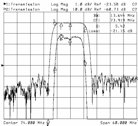
Horizontal: 6MHz/Div Vertical: 10dB/Div
