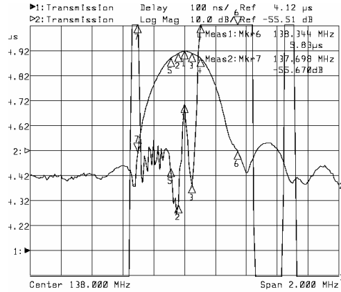
Horizontal: 0.2MHz/Div Vertical: 100nsec/Div
