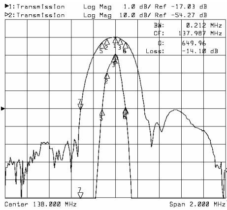
Horizontal: 0.2MHz/Div Vertical: 10dB/Div
