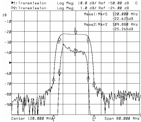
Horizontal: 8MHz/Div Vertical: 10dB/Div
