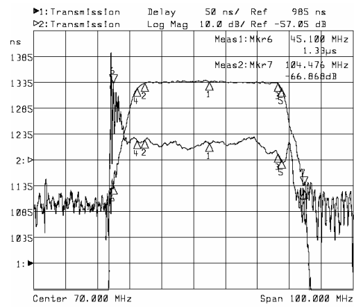
Vertical: 50nsec/Div Horizontal: 10MHz/Div
