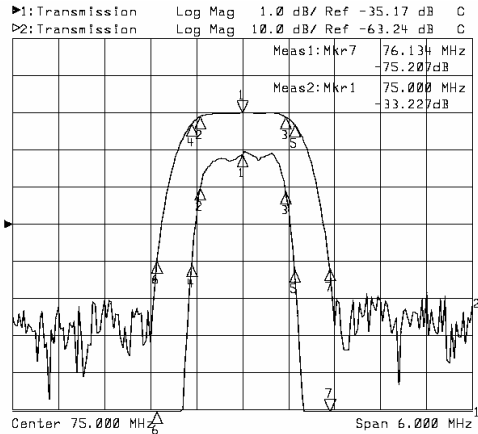
Horizontal: 0.6MHz/Div Vertical: 10dB/Div
