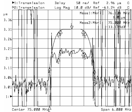
Horizontal: 0.6MHz/Div Vertical: 100ns/Div
