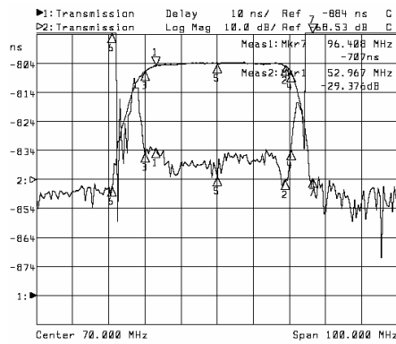
Horizontal: 10MHz/Div Vertical: 10nsec/Div
