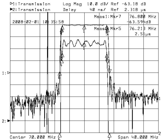
Horizontal: 4MHz/Div Vertical: 40ns/Div&10dB/Div
