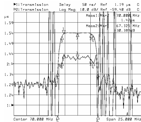
Horizontal: 2.5MHz/Div Vertical: 50nsec/Div
