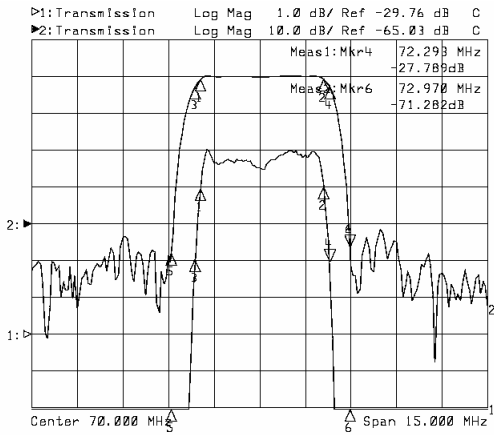
Horizontal: 1.5MHz/Div Vertical: 10dB/Div
