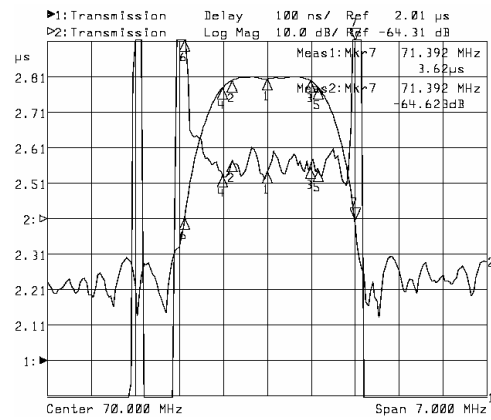
Horizontal: 0.7MHz/Div Vertical: 100ns/Div
