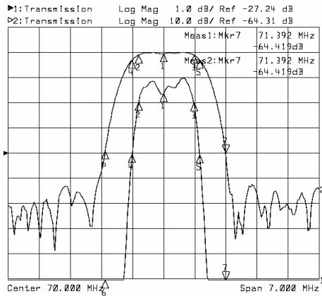
Horizontal: 0.7MHz/Div Vertical: 10dB/Div
