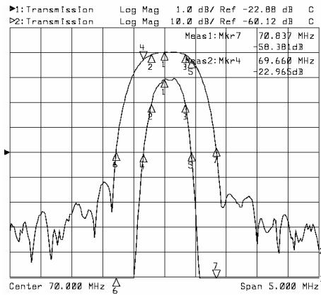
Horizontal: 0.5MHz/Div Vertical: 10dB/Div
