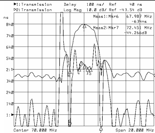
Horizontal: 2MHz/Div Vertical: 100ns/Div
