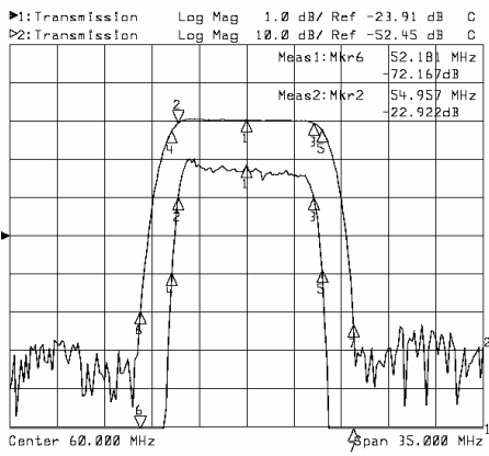
Horizontal: 3.5MHz/Div Vertical: 10dB/Div
