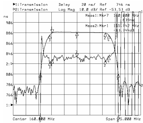
Horizontal: 2.5MHz/Div Vertical: 20nsec/Div
