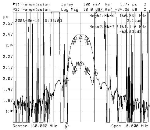
Horizontal: 1MHz/Div Vertical: 10dB/Div&100nsec/Div
