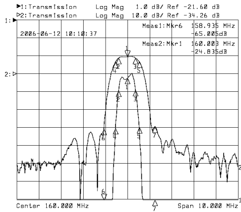
Horizontal: 1MHz/Div Vertical: 10dB/Div&1dB/Div
