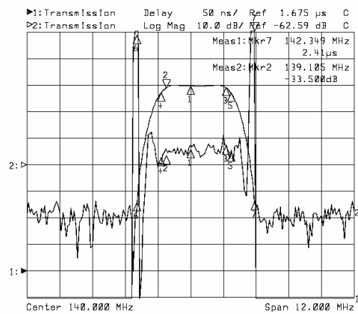
Horizontal: 1.2MHz/Div Vertical: 50nsec/Div
