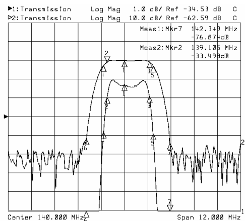
Horizontal: 1.2MHz/Div Vertical: 10dB/Div
